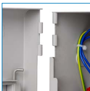
Fit the Vision Window, then re-fit both hinge pins
