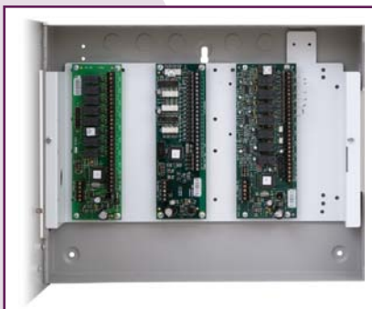
3 x I/O boards without PSU
